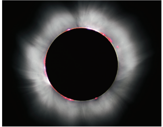
The Sun's Atmosphere (the Corona) only Visible During the Total Eclipse
